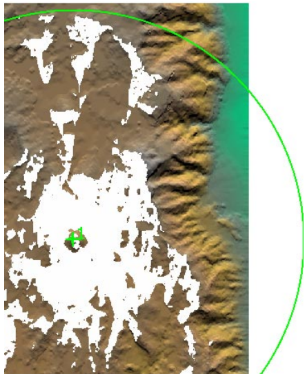
Viewshed for a viewpoint 30 meters above the ground surface.
